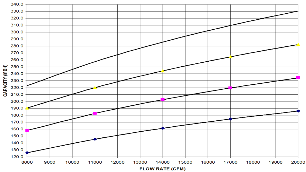
FIGURE 9 - HOT WATER COIL - 40 TON, 1 ROW, AT 40 GPM
