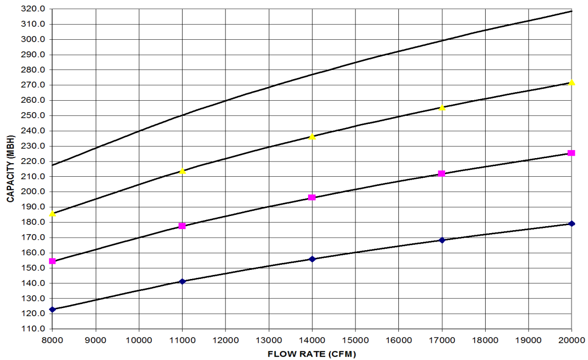
FIGURE 8 - HOT WATER COIL - 40 TON, 1 ROW, AT 30 GPM
