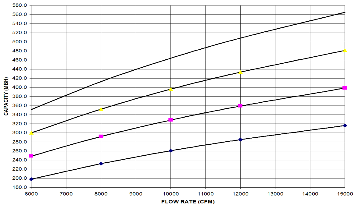
FIGURE 11 - HOT WATER COIL - 25 & 30 TON, 2 ROW, AT 40 GPM
