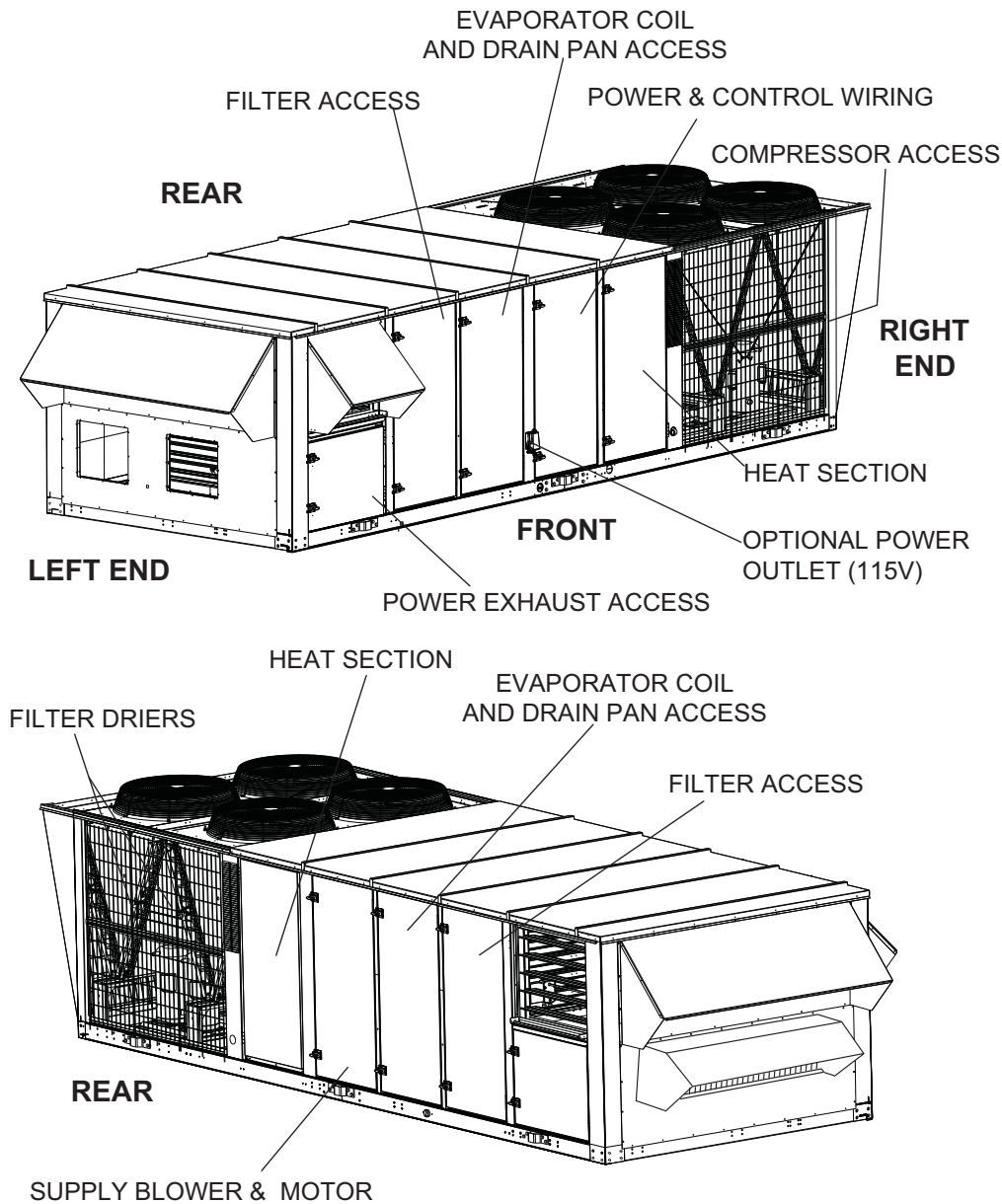
FIGURE 28 - COMPONENT LOCATION
