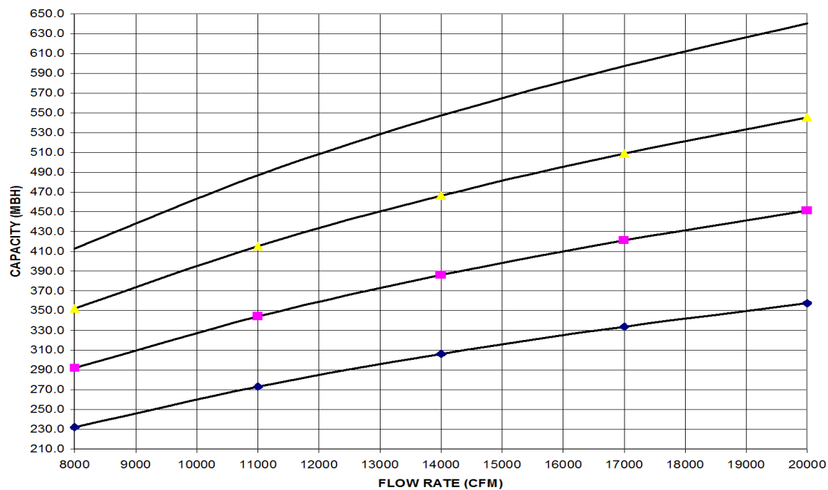
FIGURE 14 - HOT WATER COIL - 40 TON, 2 ROW, AT 20 GPM
