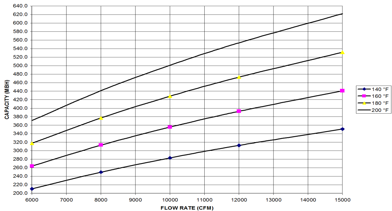
FIGURE 13 - HOT WATER COIL - 25 & 30 TON, 2 ROW, AT 80 GPM
