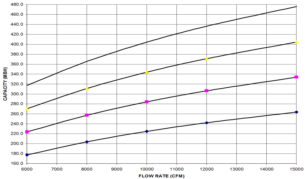
FIGURE 10 - HOT WATER COIL - 25 & 30 TON, 2 ROW, AT 20 GPM
